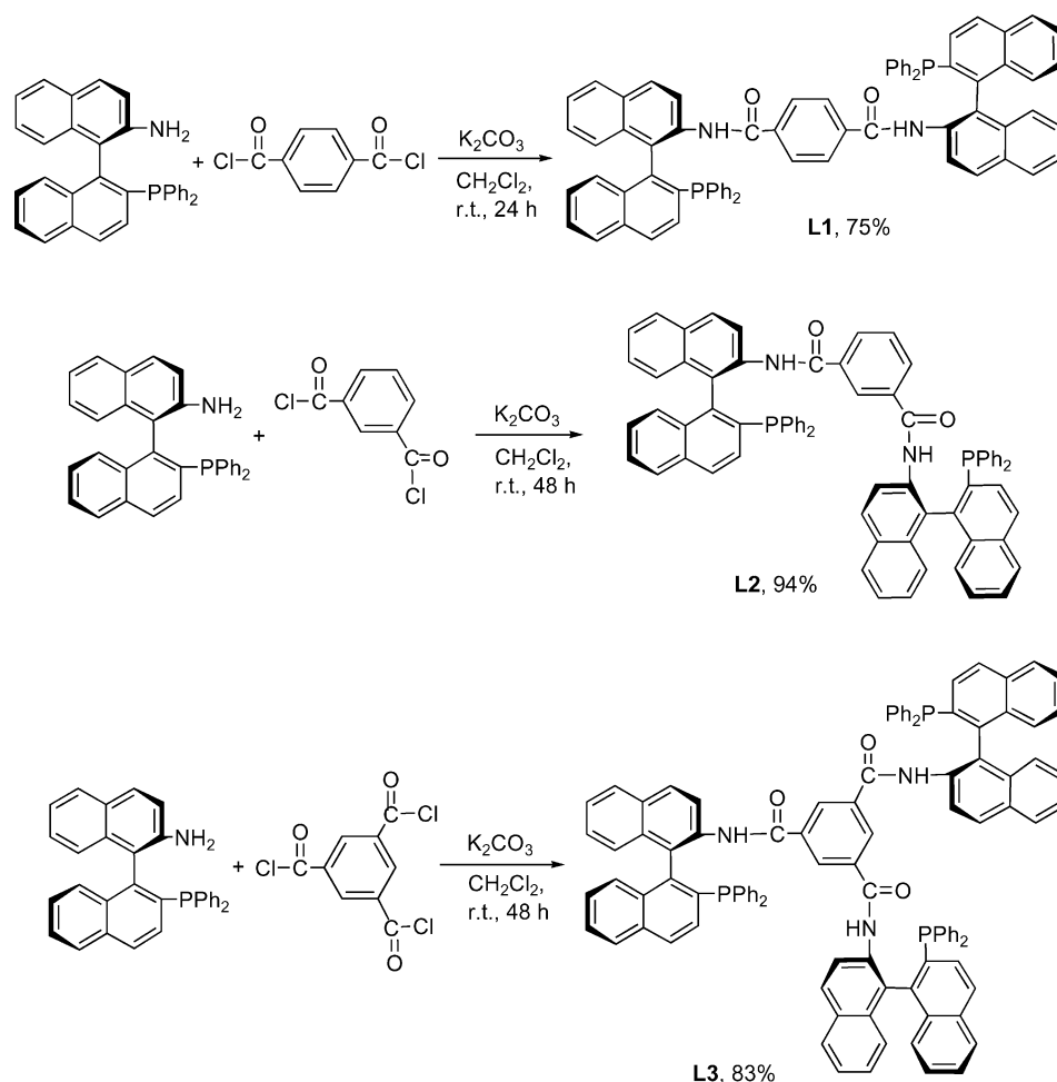
Scheme 1. Synthesis of chiral bifunctional phosphane-amide Lewis bases L1 – L3 .
