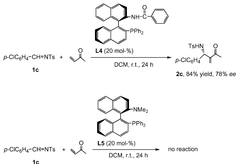
Scheme 2. Control experiments in the aza-Morita–Baylis–Hillman reaction.
